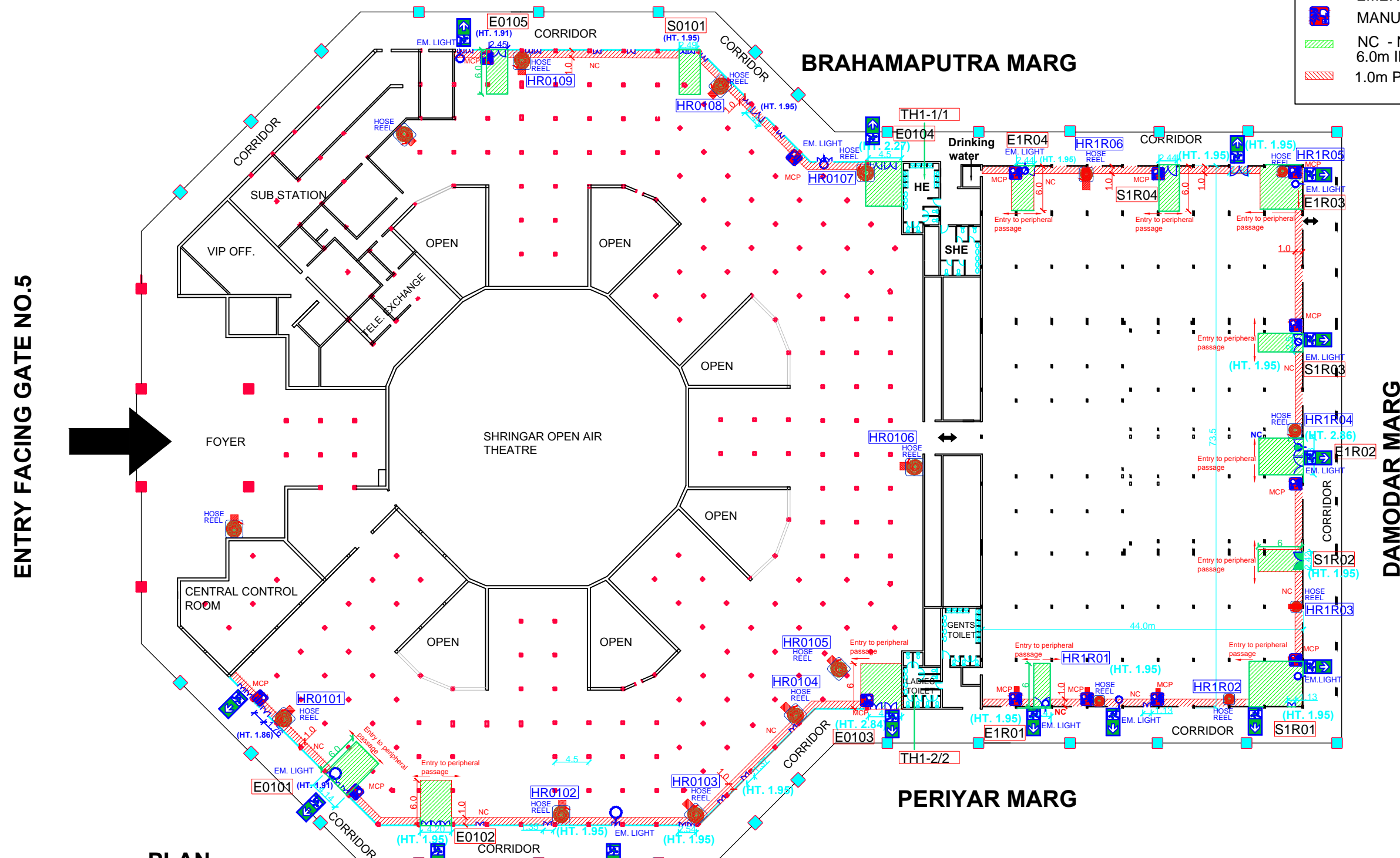
PLAN
